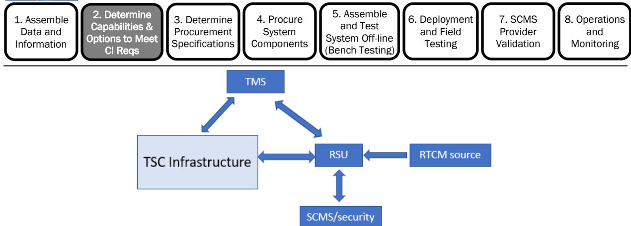
Figure 3. Illustration of a Common Connected Intersection Architecture.
