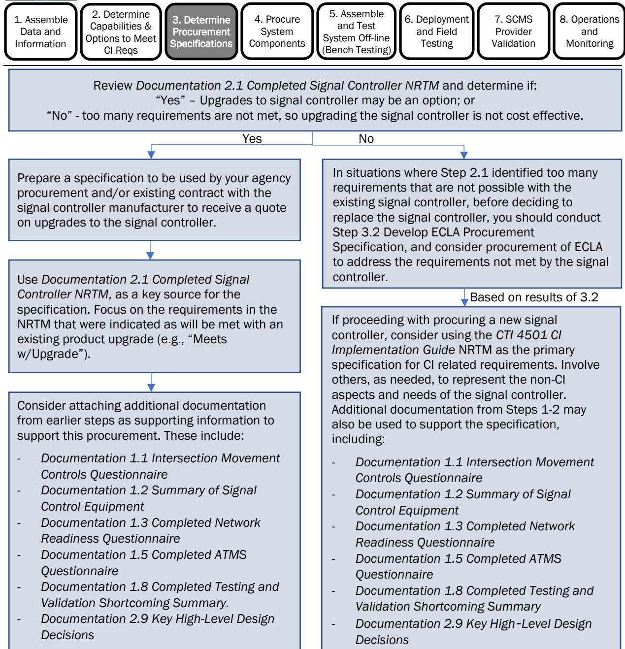
Figure 6. Flow Chart to Support Development of Procurement Specifications for Signal Controllers.
