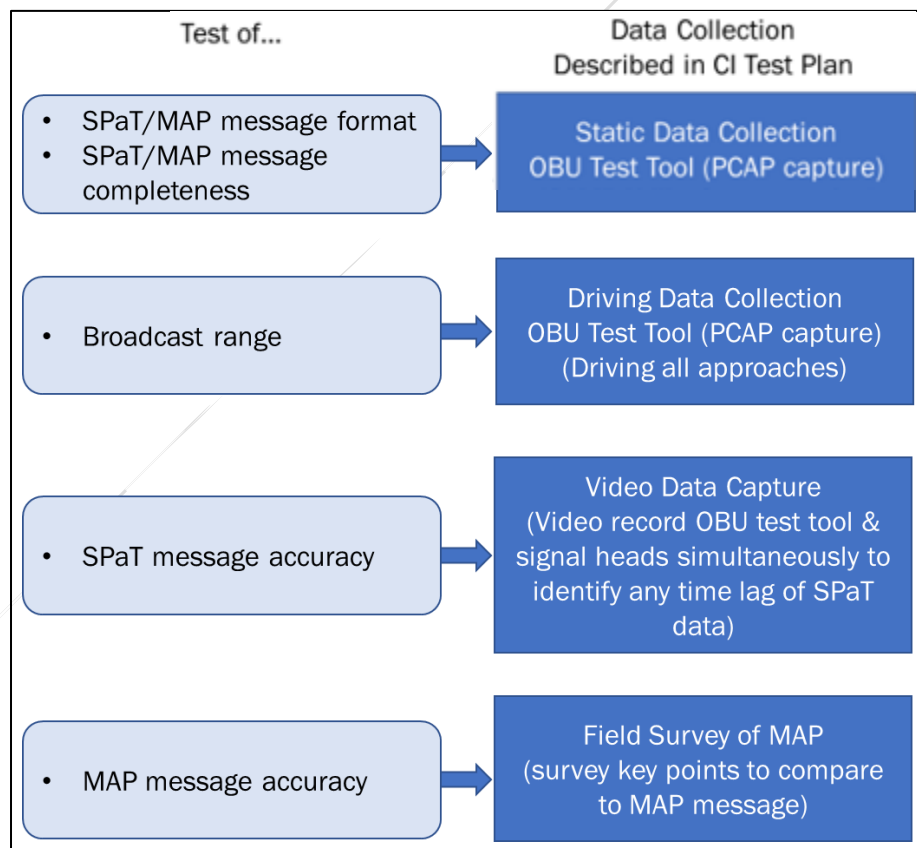
Figure 11. Data Collection Approaches to Conduct Various Tests.
