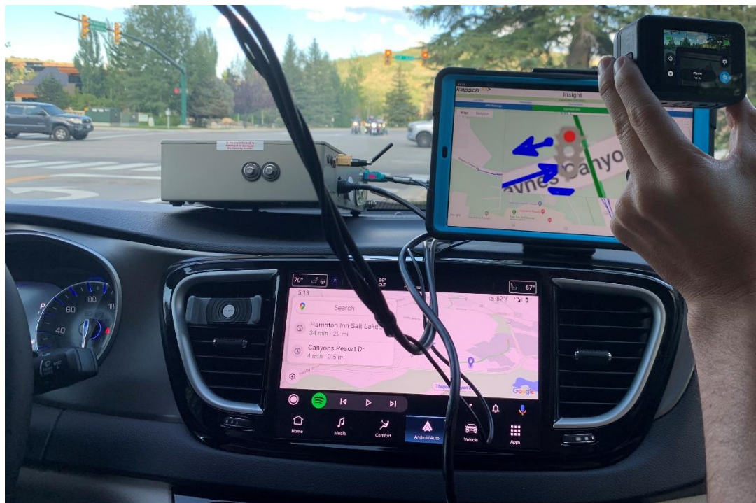
Figure 8. Testing Tools, a High-Resolution Camera, On-Board Unit, and User Interface are Some of the Test Equipment Needed to Conduct Testing and Validation Activities
